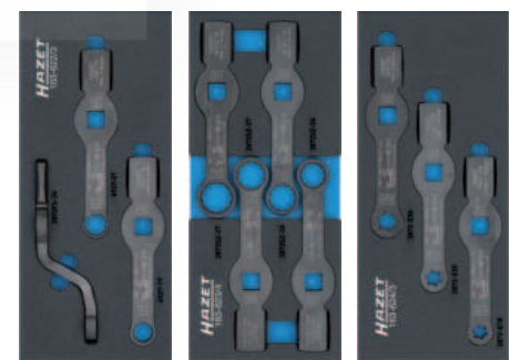
Box-end wrench set - striking face pattern 163-622/3 · 1/3+
