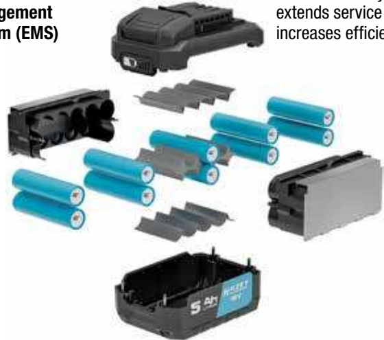
Battery with patented Thermatec® technology: integrated cooling system to extend service life
